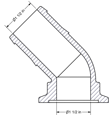
SECTION B-B SCALE 1 : 1
